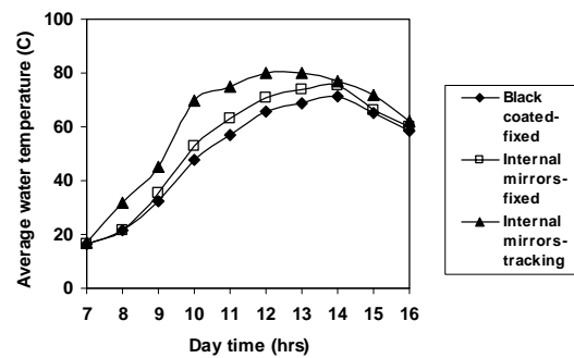
Figure 4 Average water temperature for the three proposed systems at the three working days.
