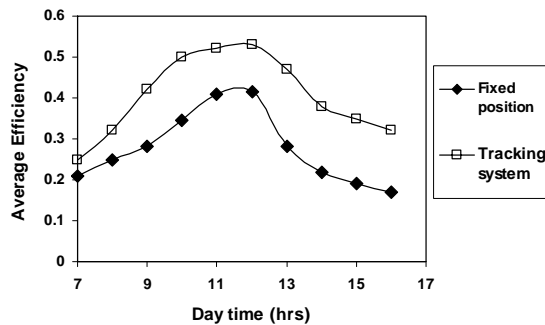
Figure 6 Average efficiency for cookers at fixed and on tracking systems for the three working days
