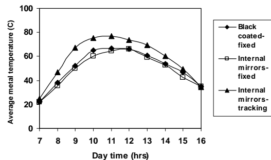
Figure 5 Average metal temperature for the three proposed systems at the three working days
