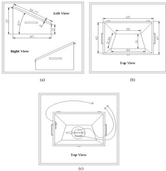
Figure 2 Three dimensional views of the designed solar cooker, (a) and (b) are cooker dimensions in cm, and (c) thermocouple connections in the cooker
