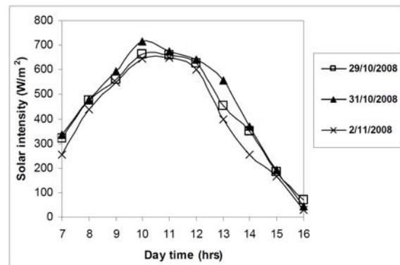
Figure 3 Solar intensities for the three working days
