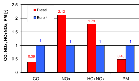
Fig. 16. Comparison of vehicle emission factor
