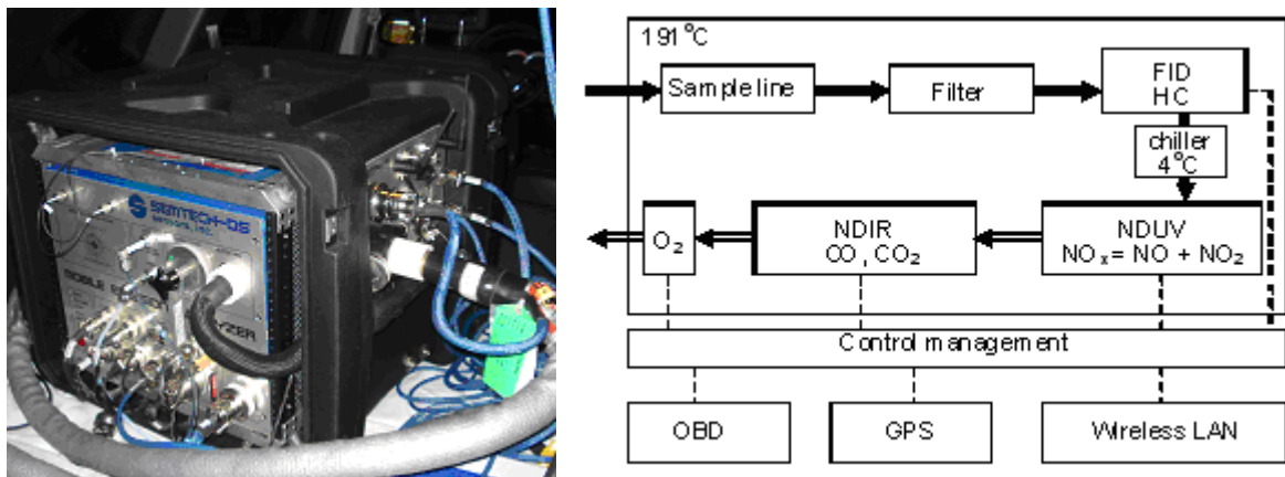
Figure 3. View and diagram of a portable analyzer; exhaust gas flow channels (==) and electrical connections circled (---)
