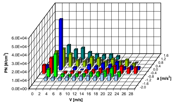
Figure 13. Particle number emission in each speed and acceleration range under city traffic conditions
